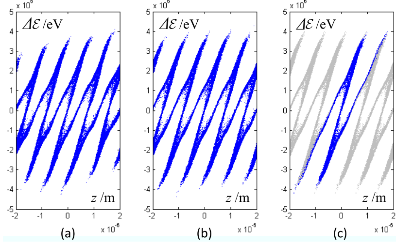
FIG. 9: Application A: longitudinal phase space direct after chicane 3. (a) Calculated with QField-non-periodic, 1E6 macro-particles, 30 fs (FWHM) laser modulation, (b) calculated with QField-non-periodic, 20E6 particles, 60 fs (FWHM) laser modulation, (c) calculated with QField-periodic.
