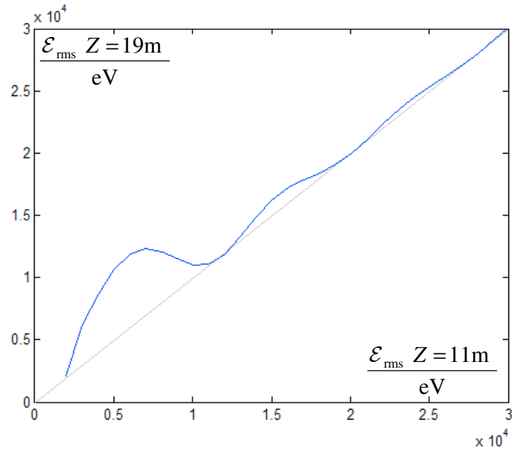
FIG. 21: Application C: energy spread at the spectrometer (position 19 m) as function of the spread directly after the laser heater chicane (position 11 m). The initial spread varies due to different laser modulation.
